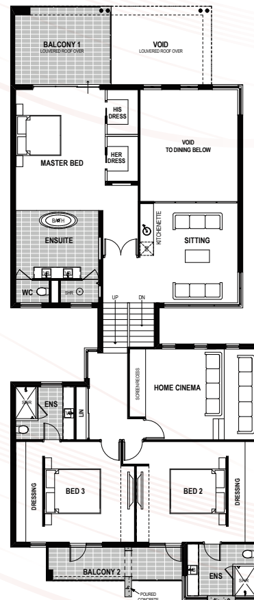
Upper floor
