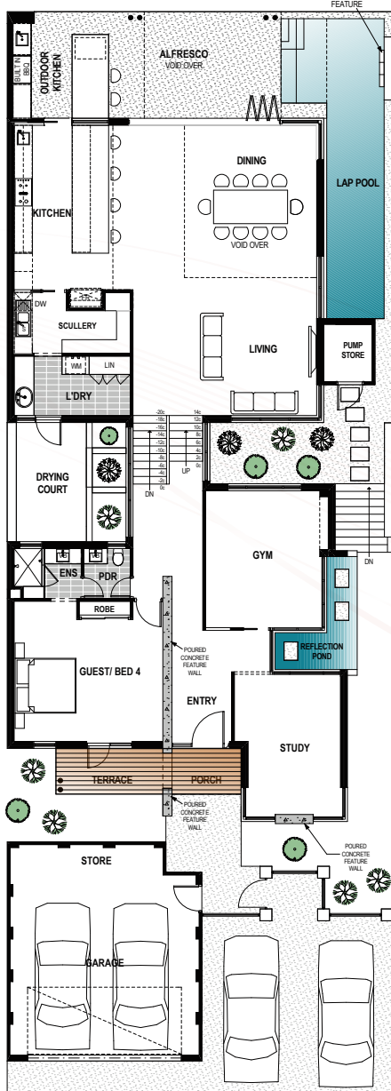
Ground floor
